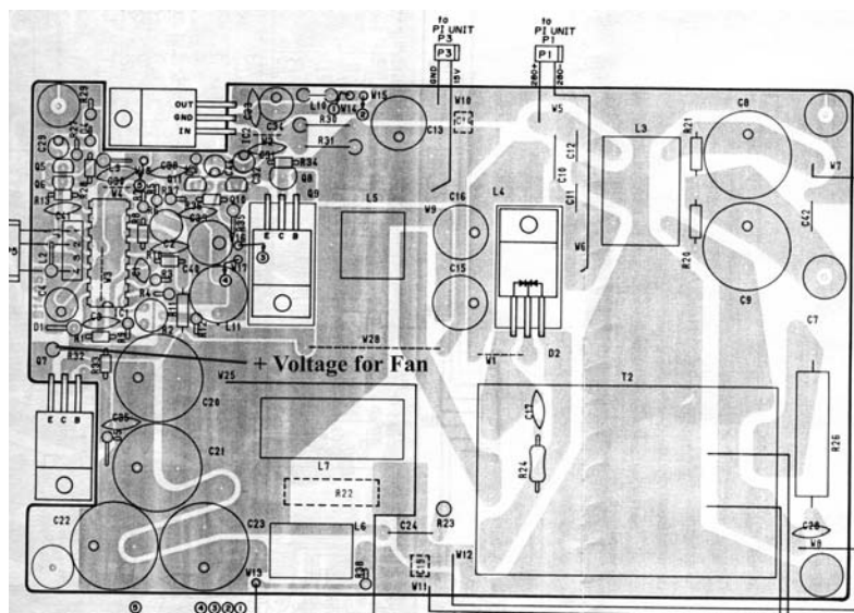
Pictorial of Power Supply Board Showing Fan Connections
