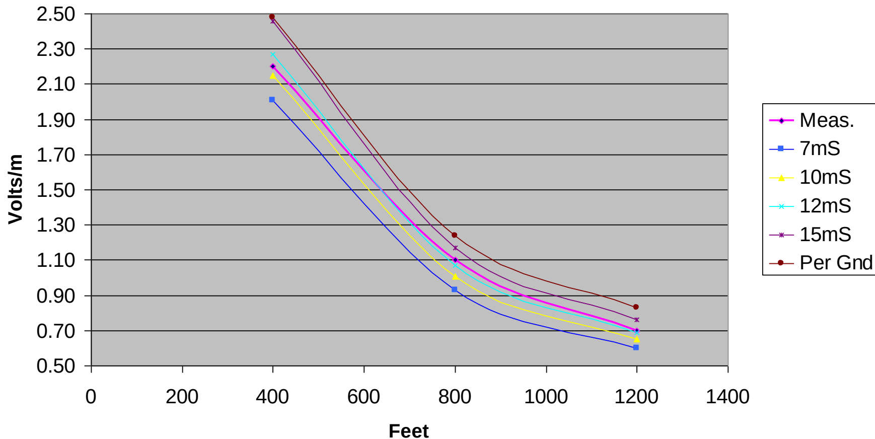
Short Range Surface Wave Intensity, Measured Vs NEC4 Predicted
